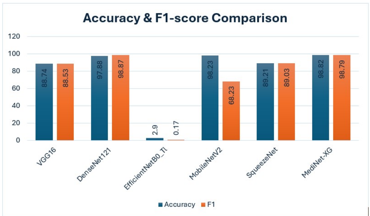
Figure 5.32: Accuracy comparison on prepared dataset[2].
