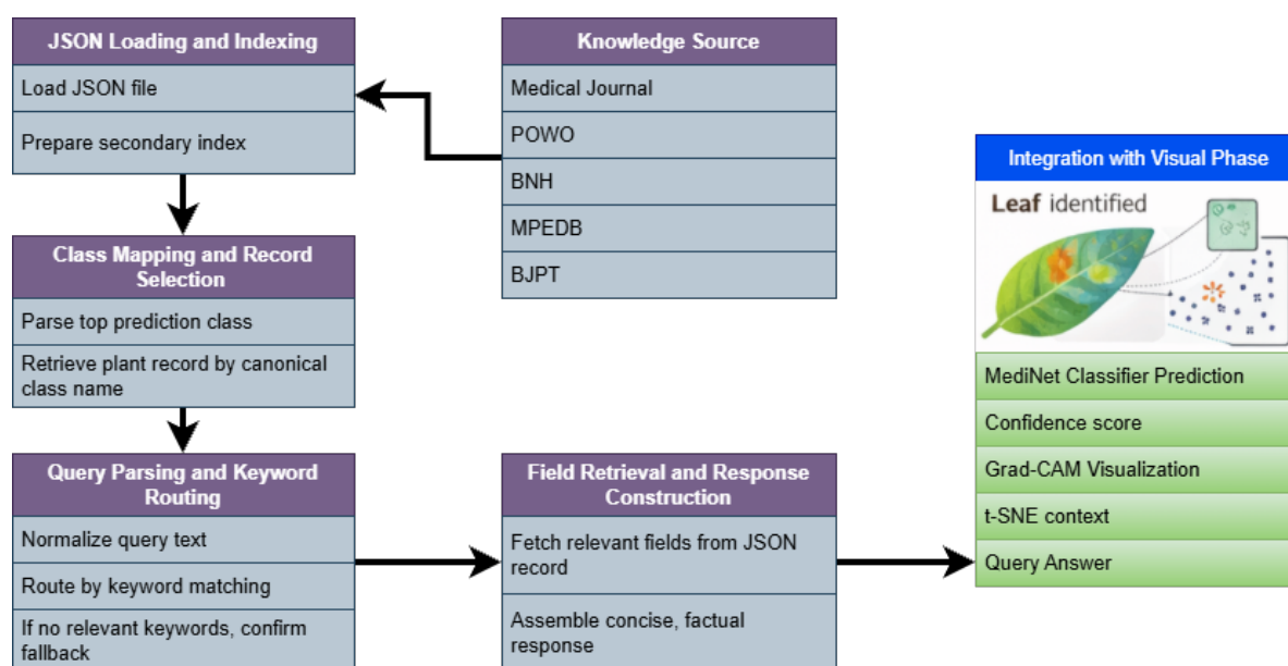
Figure 3.19: The query generator architecture.
